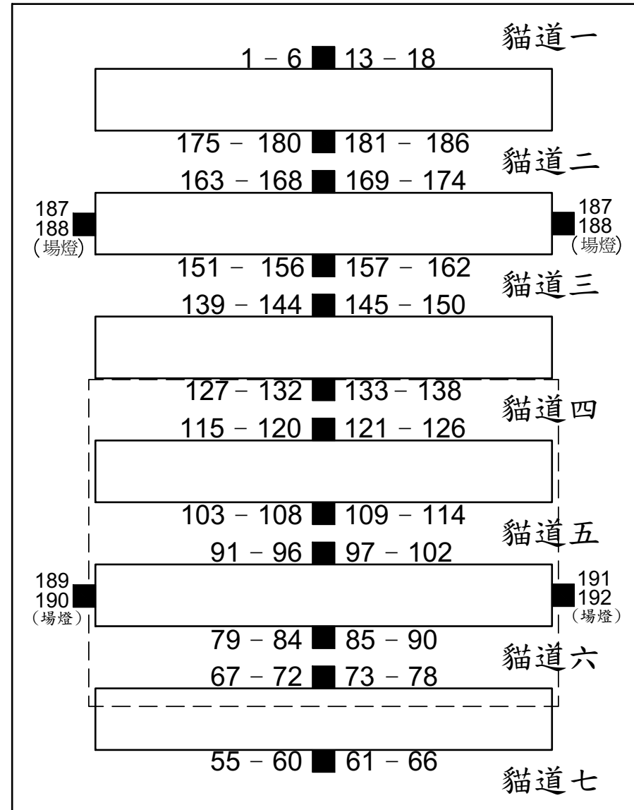
圖(九) 小表演廳_燈光迴路資訊 Figure(9) Experimental Theatre__Lighting Circuit Information
