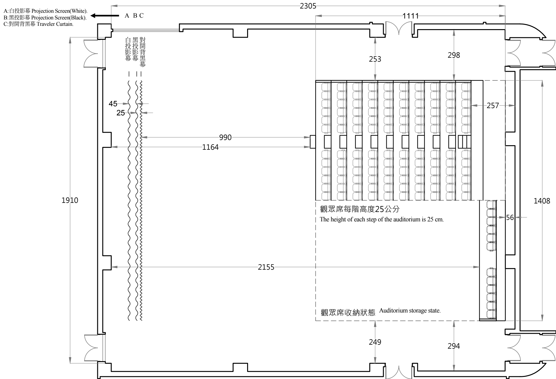
圖(二) 小表演廳_階梯式電動伸縮觀眾席示意圖(單位:公分) Figure(2) Experimental Theatre_1 st Floor Plan with Retractable Seating System (Unit: cm)
